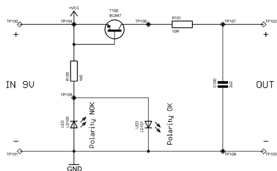
1. Input protection circuit
