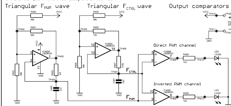
4. Two channel alternating PWM generator
