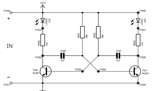
5. Astable flip-flop
