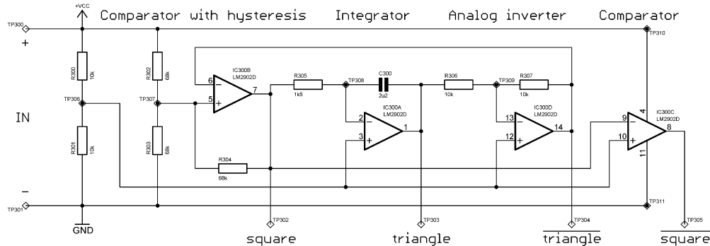
3. Square and triangular waveform generator
