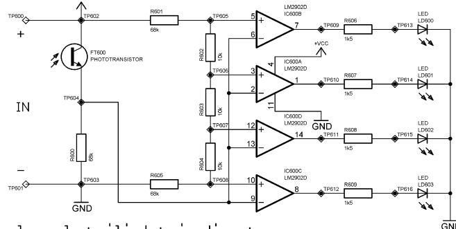
6. Four level twilight indicator
