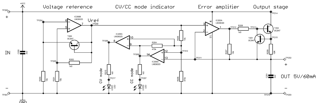
2. Fixed voltage regulator with overcurrent limiter and CV/CC mode indicator
